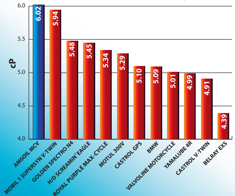
20W-50 Motorcycle Oil - High Temperature Viscosity Protection Higher values reflect better film strength. ASTM TEST METHOD D-4683 March 16, 2005
